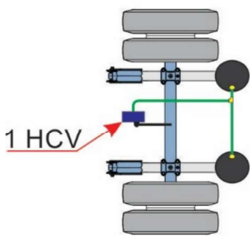
Single Axle Group
